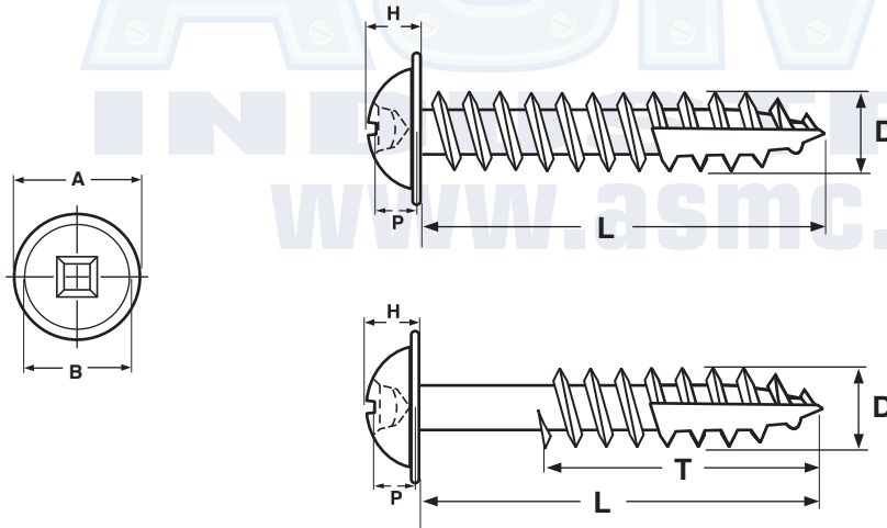
ROUND WASHER SQUARE RECESS DEEP THREAD WOOD SCREW WITH TYPE-17 POINT
