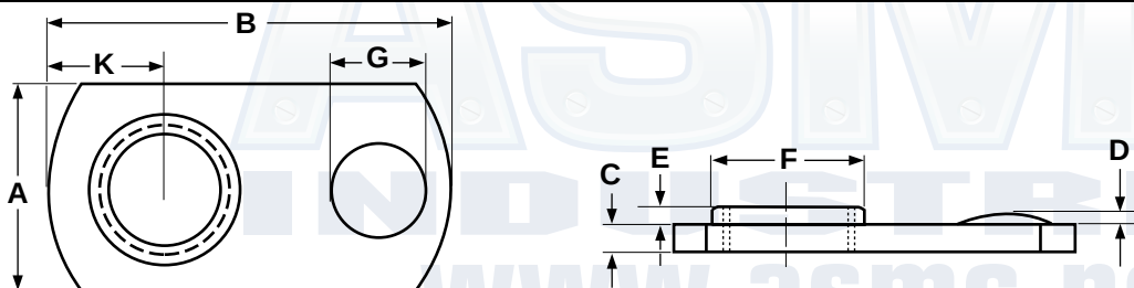
WELD NUTS - OFFSET HOLE DESIGN WITH SINGLE PROJECTION
