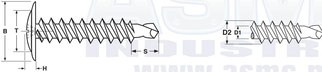
MODIFIED TRUSS HEAD PHILLIPS SELF DRILLING SCREWS
