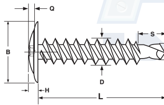
Six-Lobe Recess
