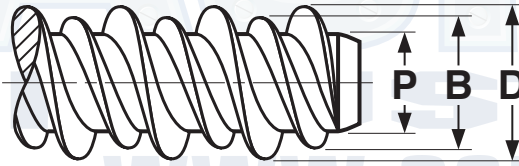
THREAD AND HOLE DIMENSIONS FOR HIGH-LOW THREAD FORMING SCREWS
