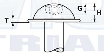
Round Washer Six-Lobe
