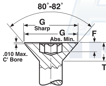
SIX-LOBE DRIVE FLAT HEADS
