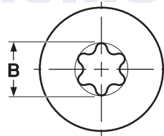
SIX-LOBE DRIVE FLAT UNDERCUT HEADS
