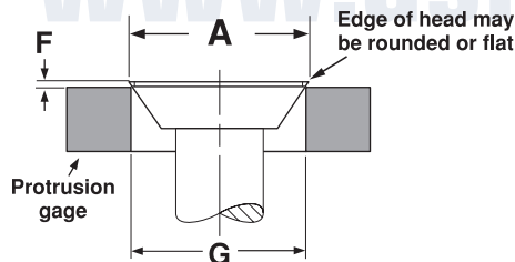
SIX-LOBE DRIVE FLAT UNDERCUT HEADS
