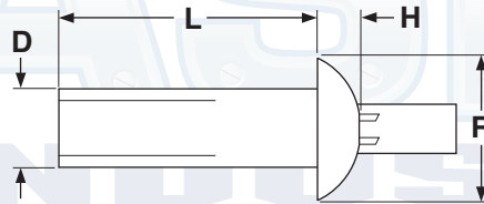
UNIVERSAL HEAD DRIVE PIN RIVETS
