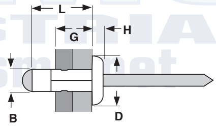
DOME HEAD
