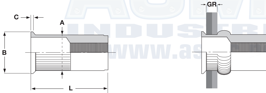
RIBBED BODY, SMALL FLANGE BLIND THREADED INSERTS
